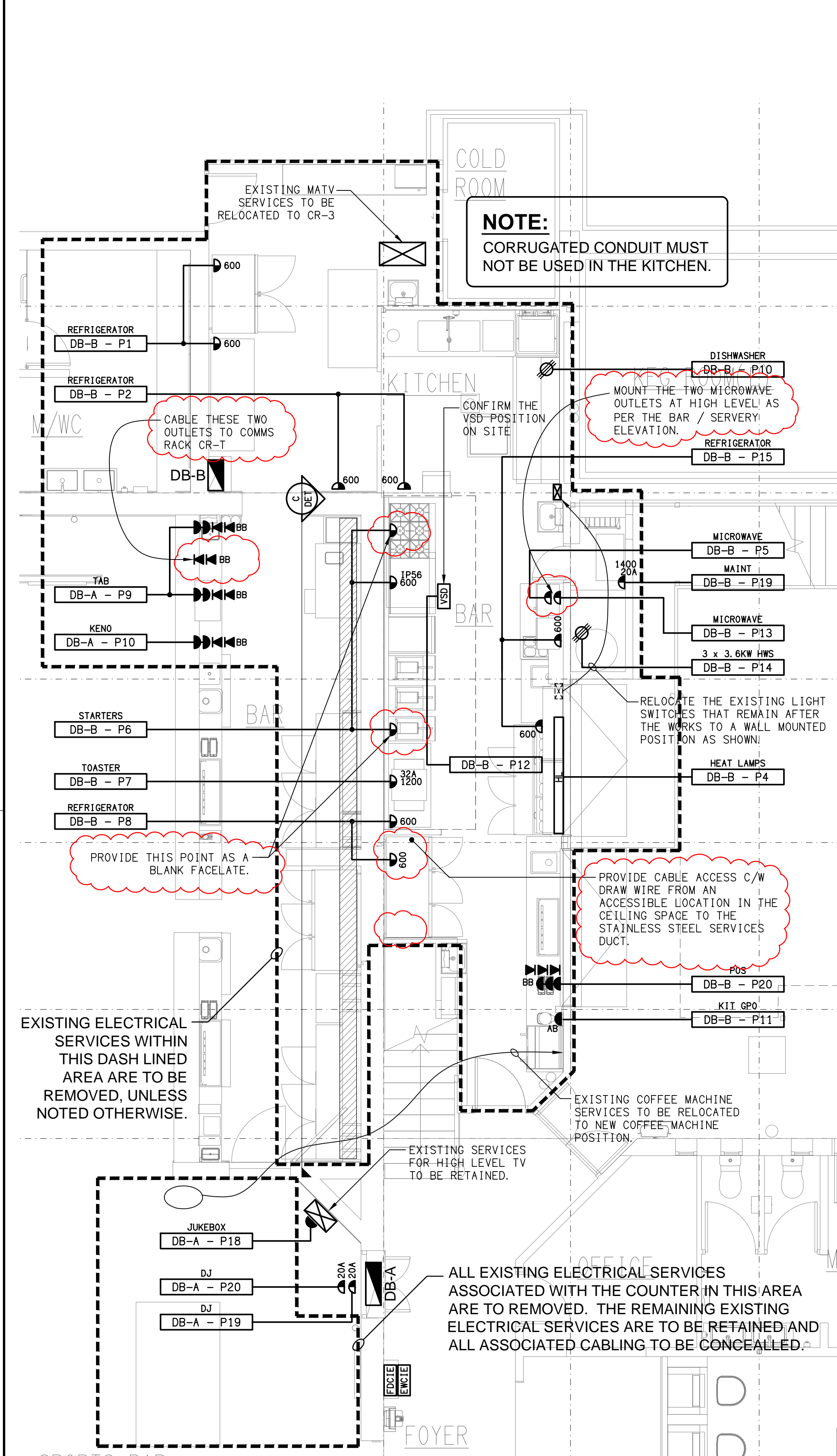
DETAIL A KITCHEN & BAR FLOOR PLAN SCALE 1:50
